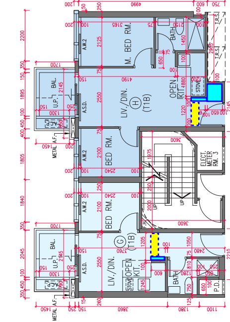
PART PLAN AT 23/F & 25/F
