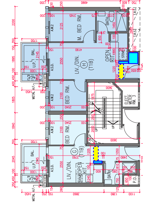
PART PLAN AT 23/F & 25/F
