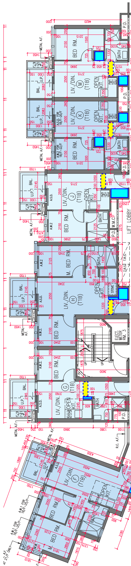
PART PLAN AT 23/F & 25/F
