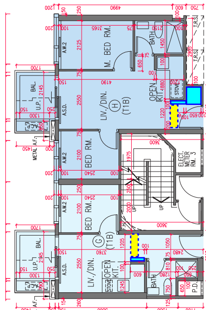
PART PLAN AT 22/F
