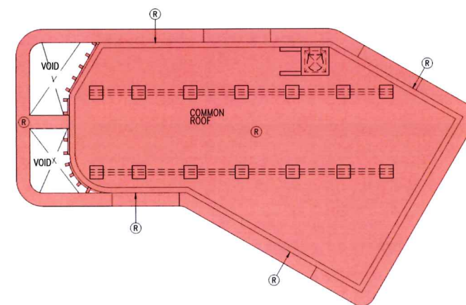
TOWER 2 TOP ROOF PLAN
