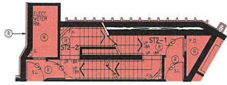
PART PLAN AT 23/F
