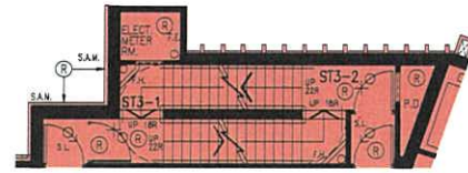
PART PLAN AT 26/F
