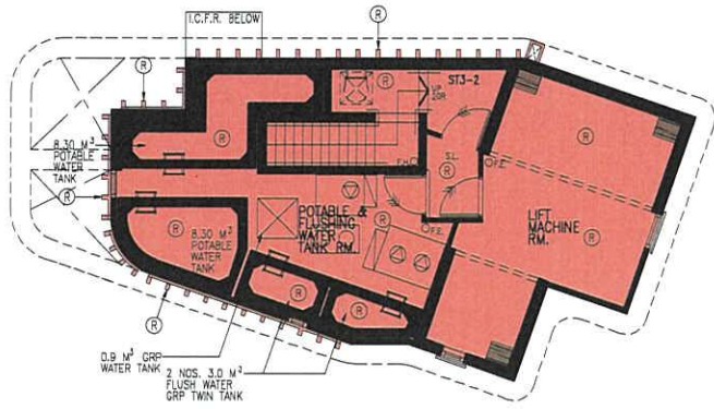
TOWER 3 UPPER ROOF PLAN
