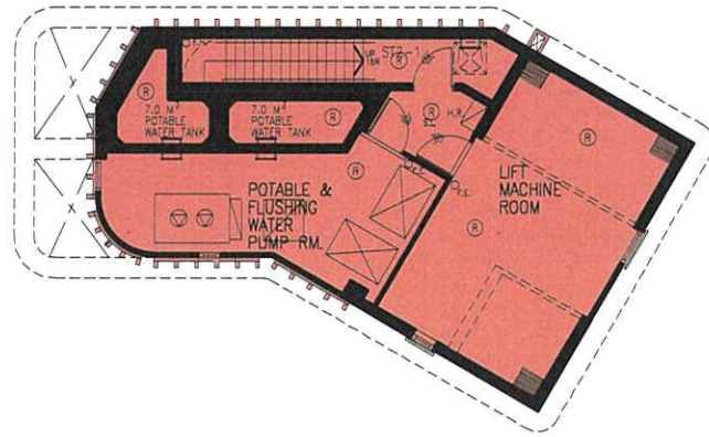
TOWER 2 UPPER ROOF PLAN
