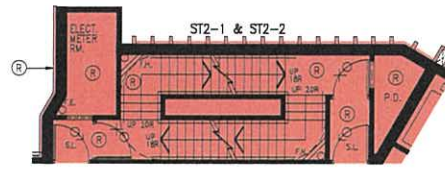
PART PLAN AT 26/F
